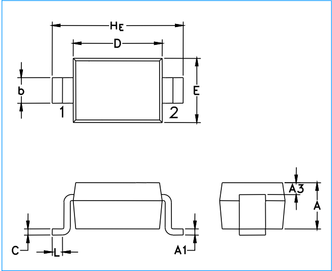
SOD-323 Package Outline & Dimensions
