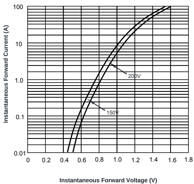
FIG3: Forward Voltage
